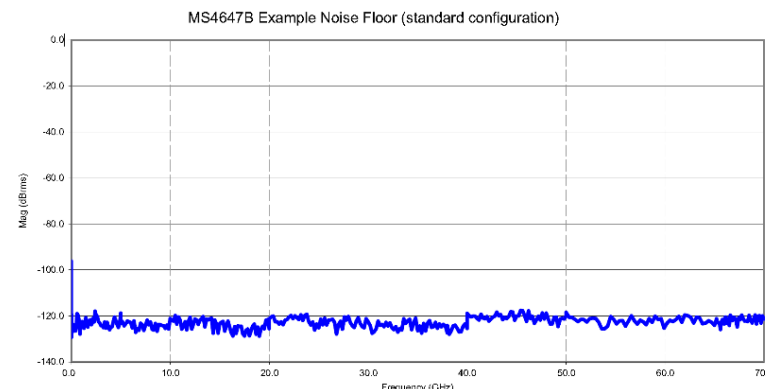
VectorStar Dynamic Range from 70 kHz to 70 GHz
